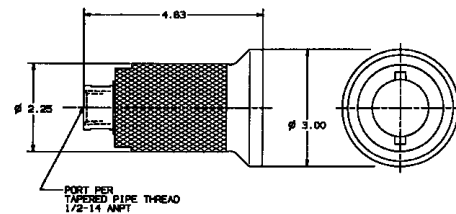
Nozzle 50E722
